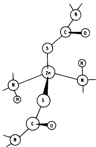
Fig. 3. Coordination geometry and bonding in \text{Zn}(\text{Pipmtc})_2(\text{Pip})_2 .
