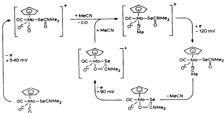
Fig. 7. Electrochemical properties of [\text{Mo}(\text{XOCNMe}_2)(\text{CO})_3(\eta^5\text{-C}_5\text{H}_5)] ( \text{X} = \text{S, Se} ). Although monoselenocarbamate is shown in the figure, the scheme applies equally well to the monothiocarbamate. (Reproduced with permission from ref. 39.)
