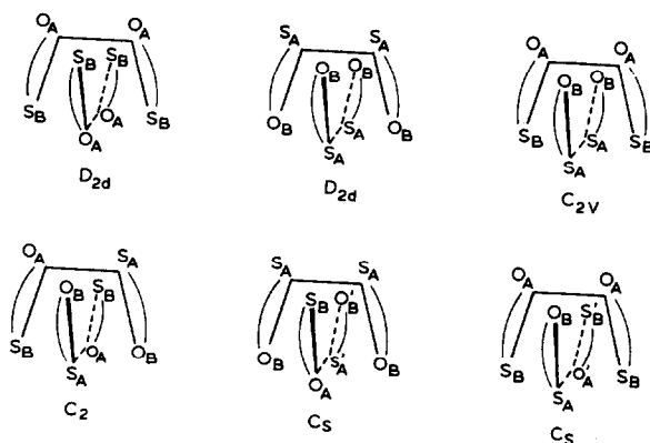
Fig. 3. Coordination geometry and bonding in \text{Zn}(\text{Pipmtc})_2(\text{Pip})_2 .
